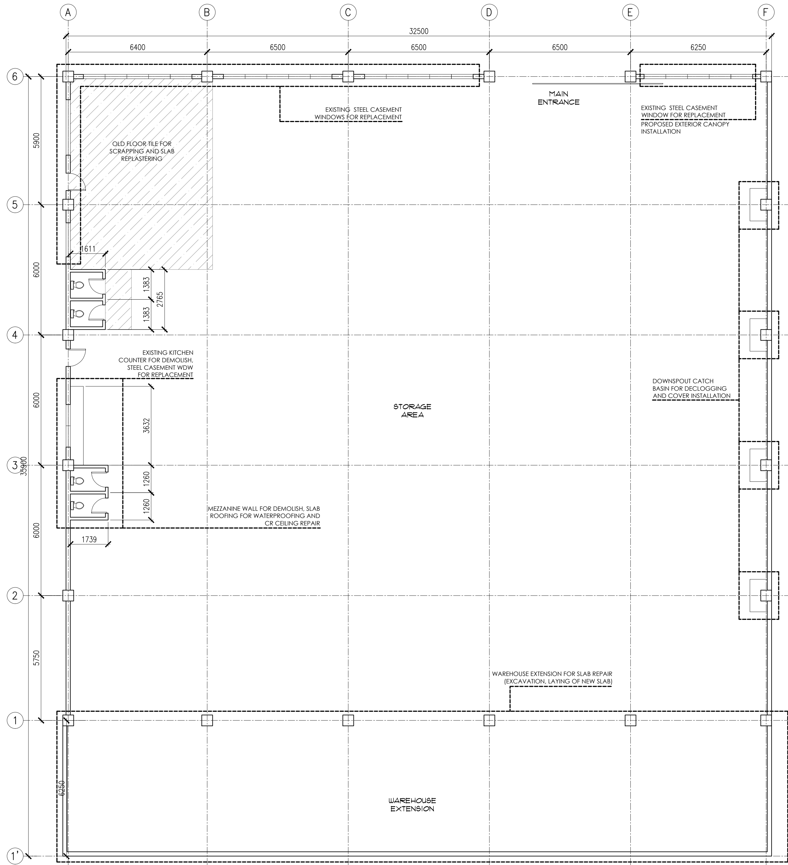
1 EXISTING FLOOR PLAN SCALE 1:100
